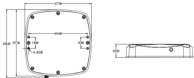
XC-AF802-BEN-B Type antenna appearance dimension drawing
