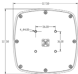
XC-AF802-BEN-A Type antenna appearance dimension drawing
